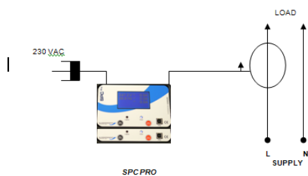
SINGLE PHASE CONNECTION
