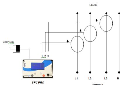
THREE PHASE CONNECTION
